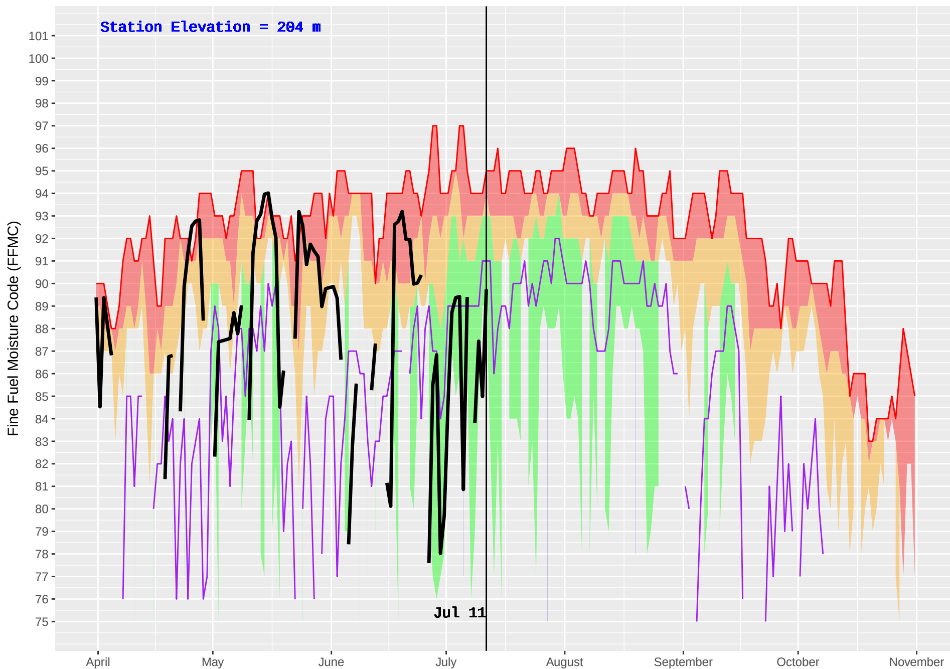
PEMBERTON BASE (301) : Historical (2001–2016) and Current (2018) Noon Fine Fuel Moisture Code (FFMC)
