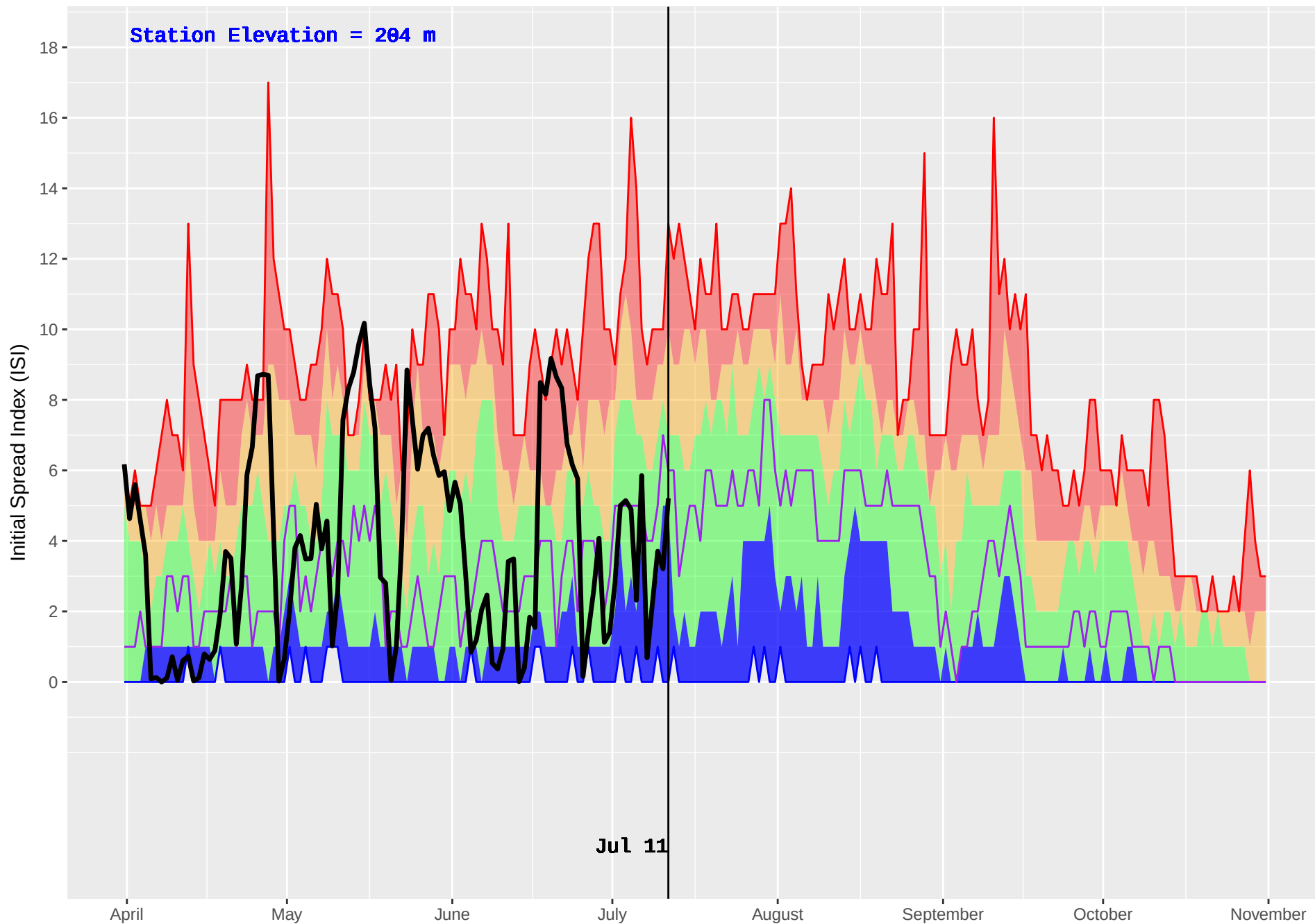
PEMBERTON BASE (301) : Historical (2001–2016) and Current (2018) Noon Initial Spread Index (ISI)
