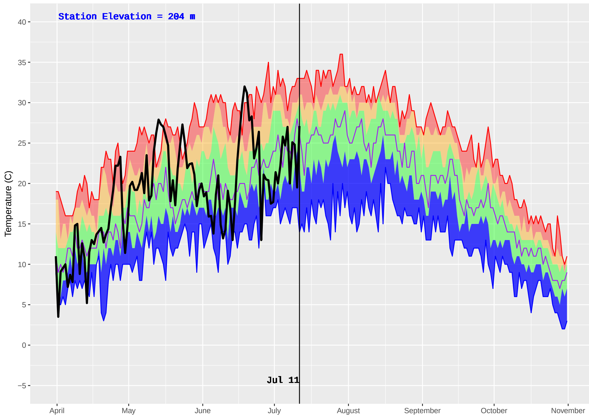
PEMBERTON BASE (301) : Historical (2001–2016) and Current (2018) Noon Temperature
