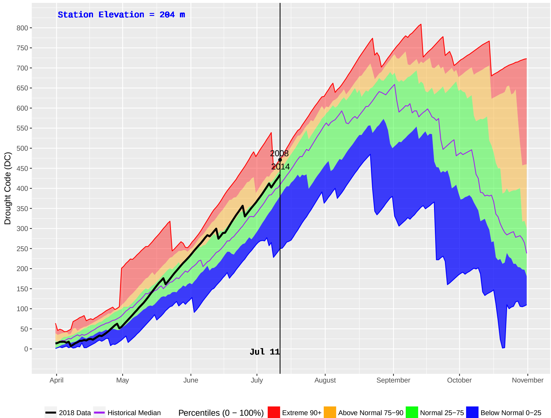
PEMBERTON BASE (301) : Historical (2001–2016) and Current (2018) Noon Drought Code (DC)
