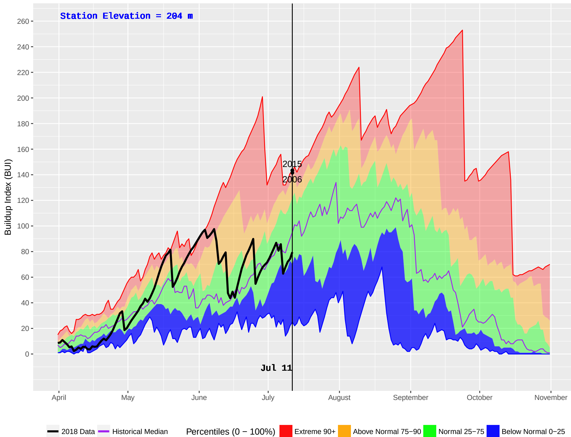
PEMBERTON BASE (301) : Historical (2001–2016) and Current (2018) Noon Buildup Index (BUI)
